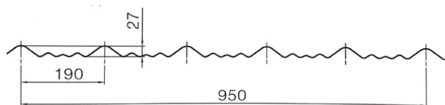
Tile Profile
